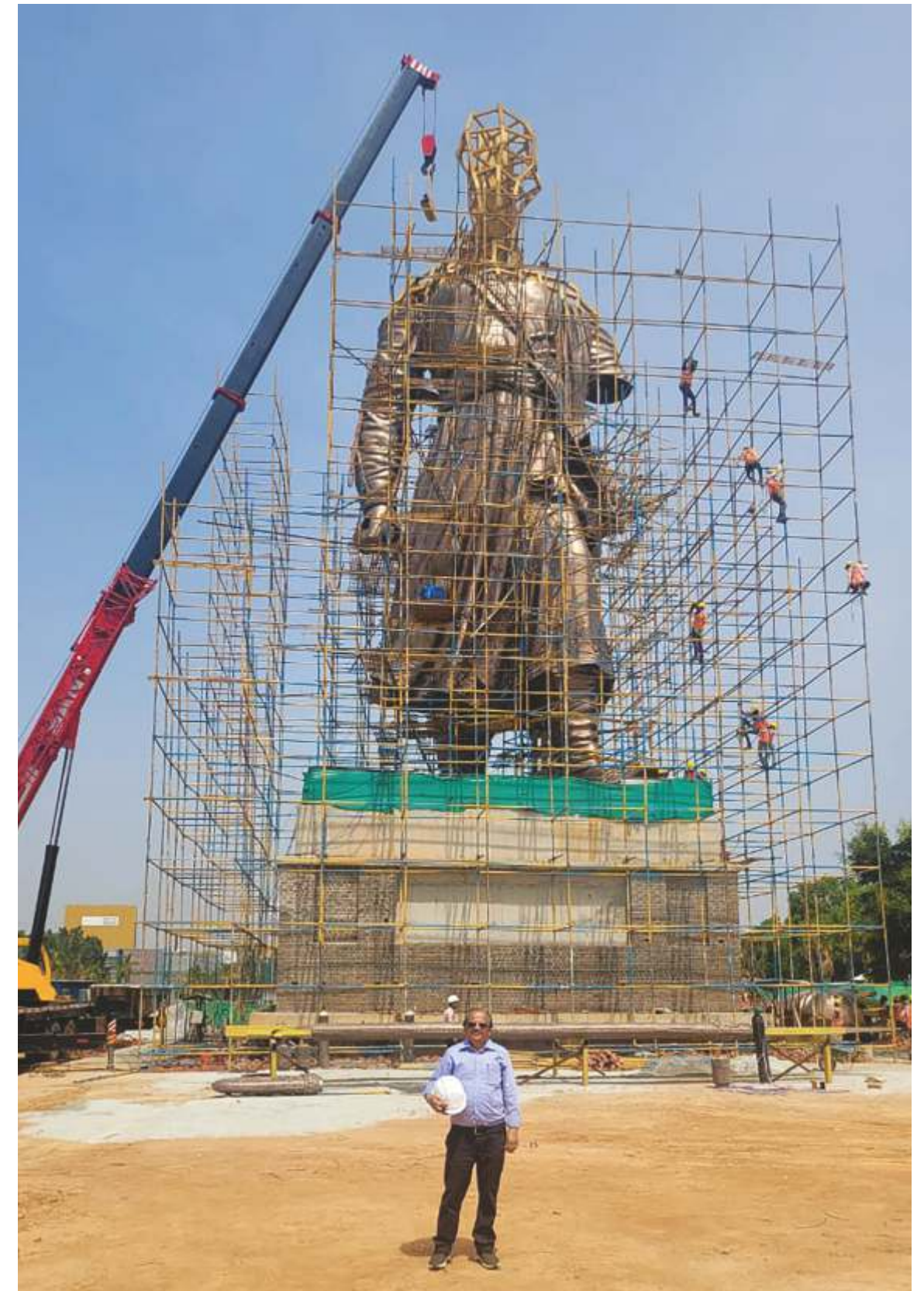
During installation of Bronze cladding on steel structure at site
